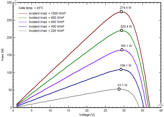
Power under different irradiation conditions
